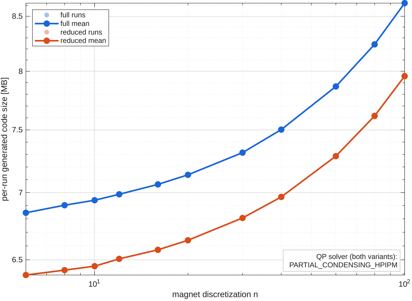
Generated C code size vs n
